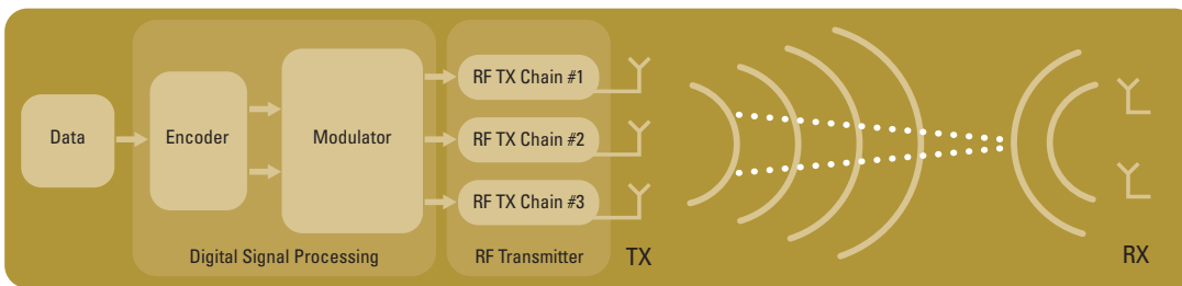
Figure 2: Transmit Beamforming
