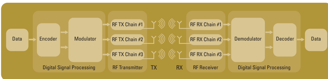
Figure 3: Multiple Transmit Chains and Multiple Receive Chains
